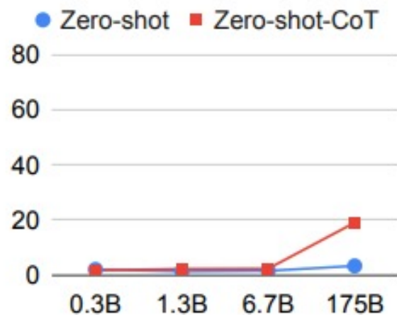
(a) MultiArith on Original GPT-3
