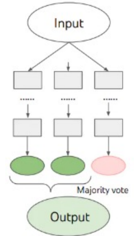
(c) Self Consistency with CoT ( CoT-SC )
